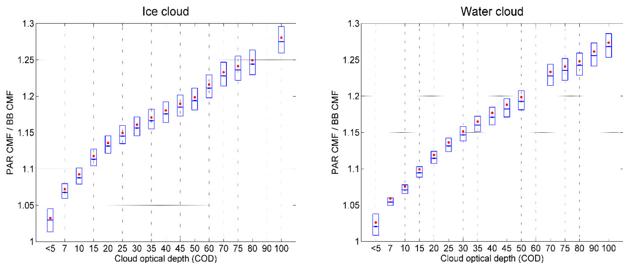
Figure 2. Simulation results of the ratio of PAR CMF to BB CMF for ice clouds ( left ) and water clouds ( right ) as function of cloud optical depth. The mean values of the boxes are marked with a red dot. The 1st, 2nd, and 3rd quartiles are marked with a blue line.
