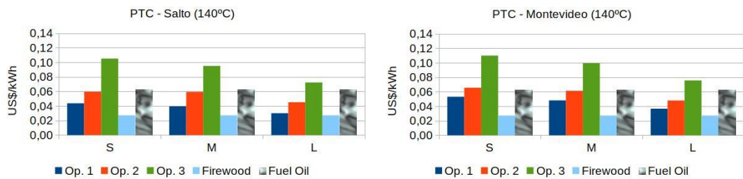
Fig. 11: LCOH of Solar Thermal Energy of PTC fields in Salto (left) and Montevideo (right), working at a mean temperature of 140^{\circ}\text{C} , with r=12\% and T=10 years. Effective prices of Firewood and Fuel are included. The options 1,2 and 3 indicate the different possible situations of tax exemptions described in 3.4.
