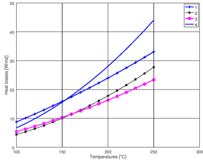
Fig. 5: Heat losses curves for LFT Technologies from Tab. 3.
